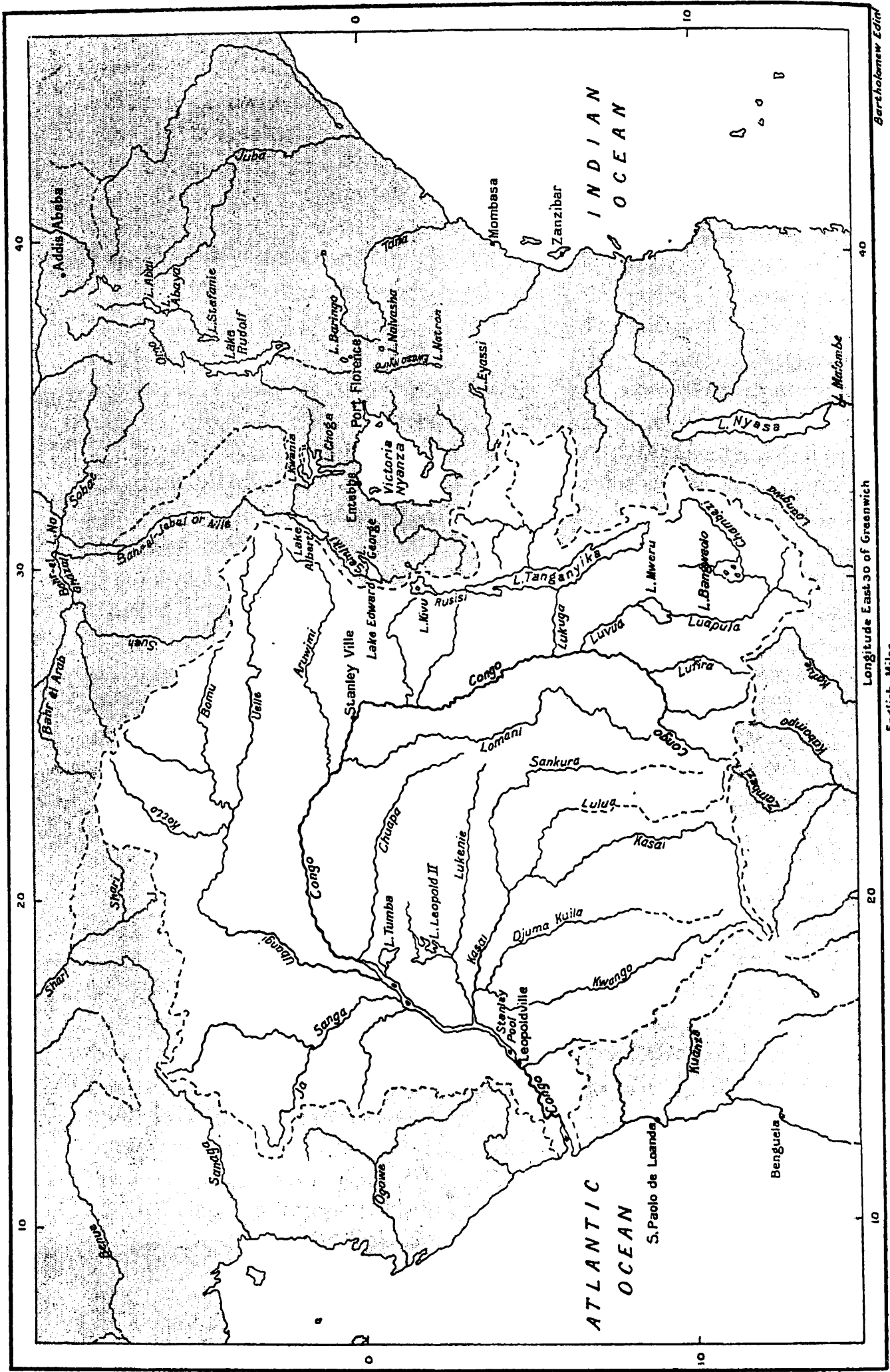
FIG. 74.—River Congo drainage basin.
