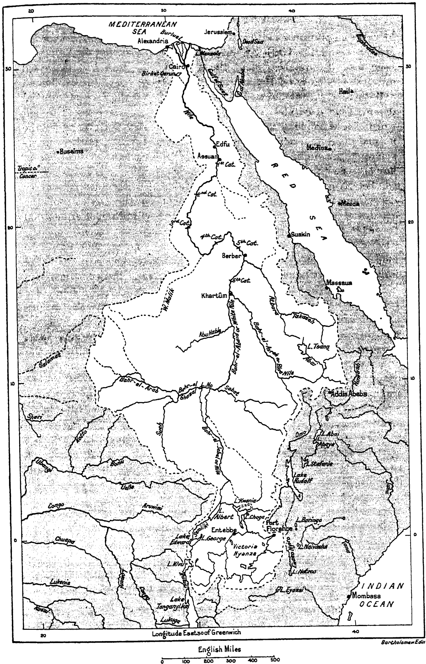
FIG. 73. — River Nile drainage basin.
