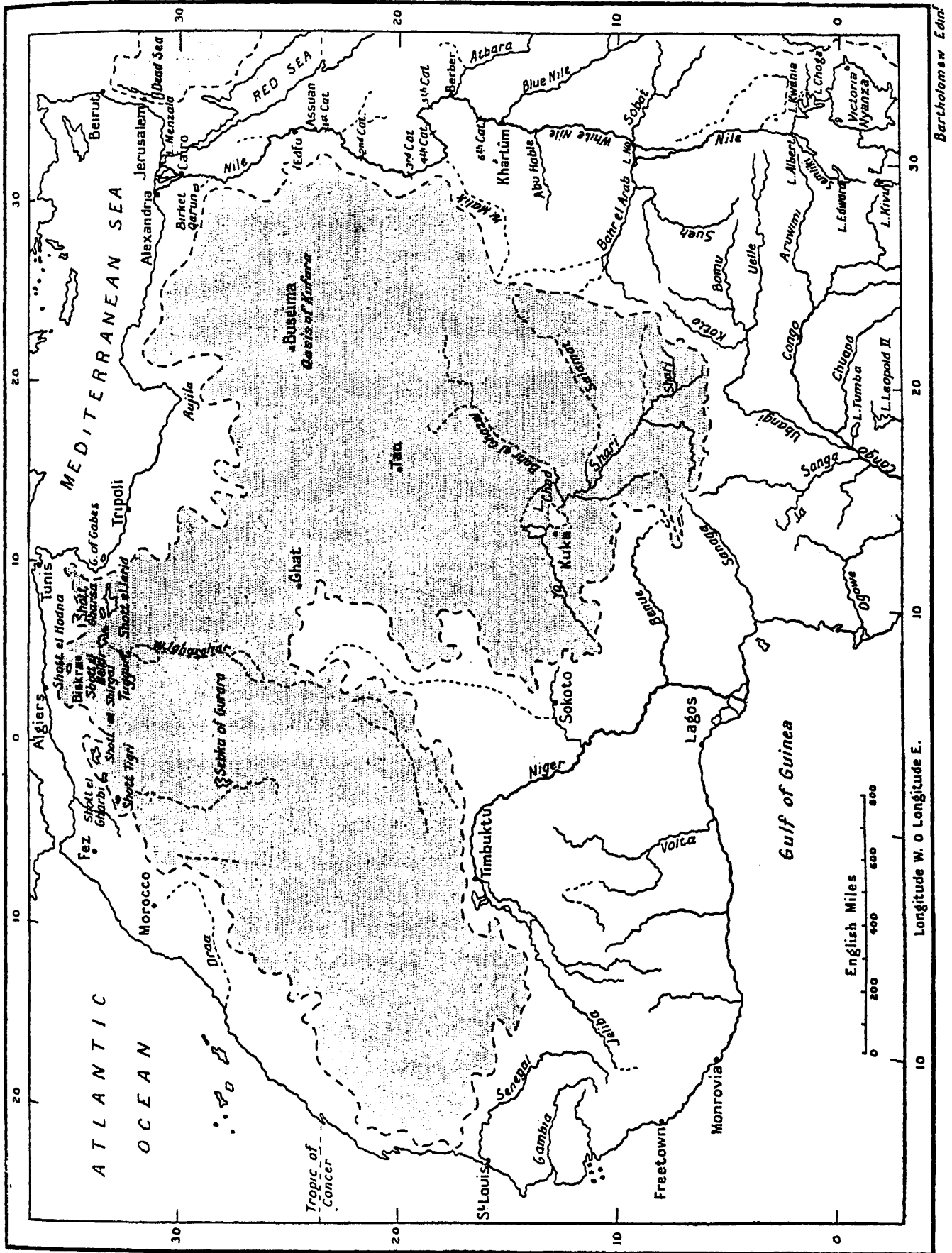
FIG. 65.—In-land drainage area of Northern Africa (Sahara and Sudan). [The inland drainage areas are stippled.]
