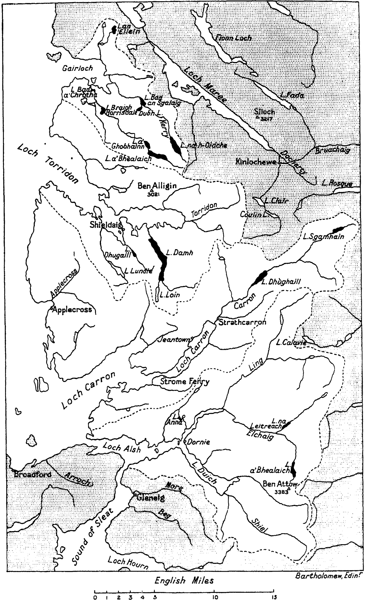
FIG. 4.—INDEX MAP OF THE GAIRLOCH, TORRIDON, CARRON, AND ALSH BASINS.
